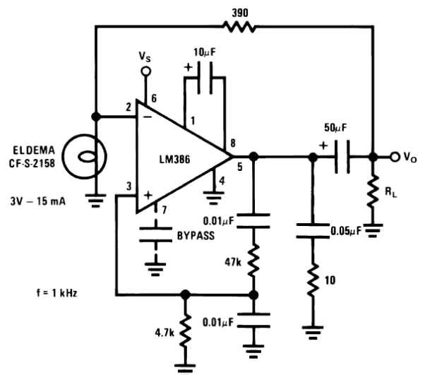
Low Distortion Power Wienbridge Oscillator
