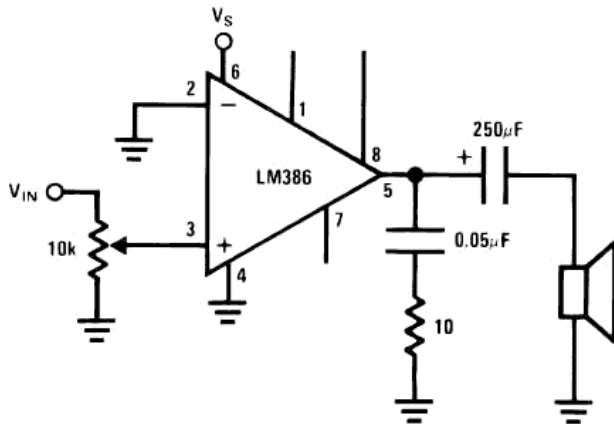
Amplifier with Gain = 20 Minimum Parts
