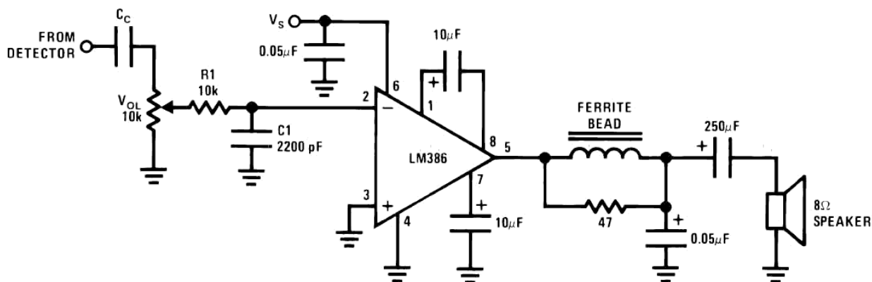
AM Radio Power Amplifier
