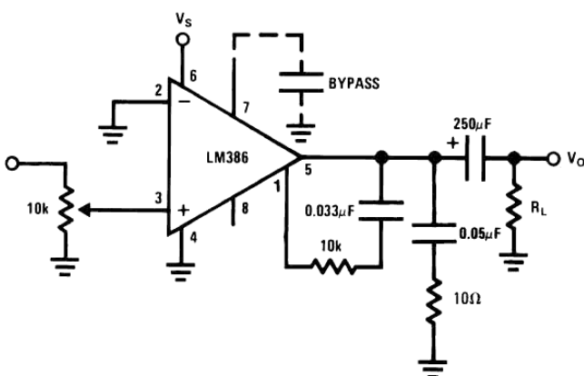
Amplifier with Bass Boost
